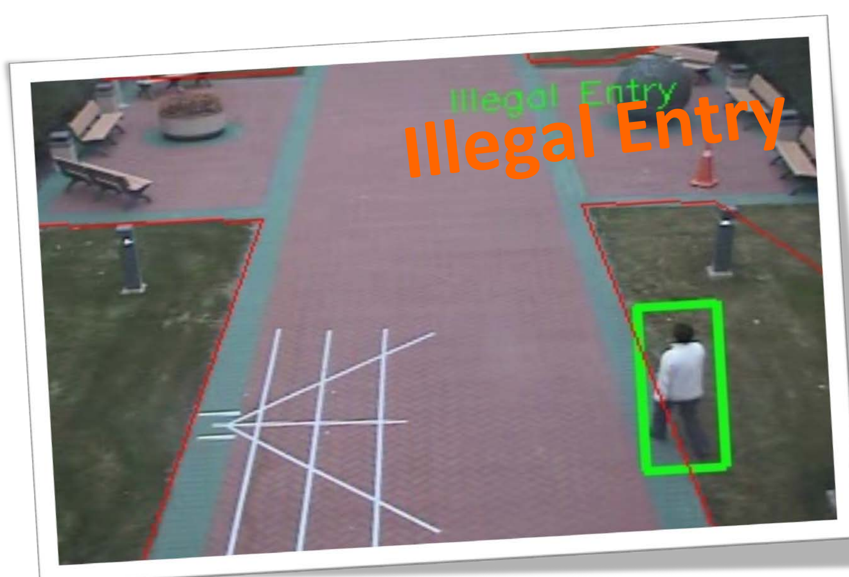
Event Detection
