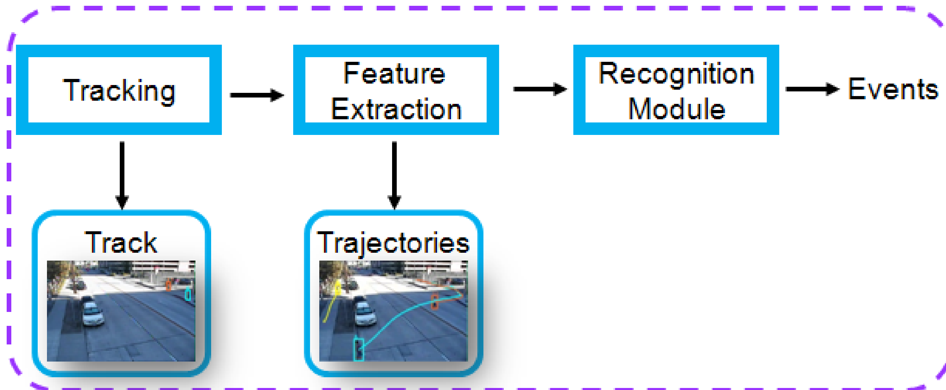
Event Detection
