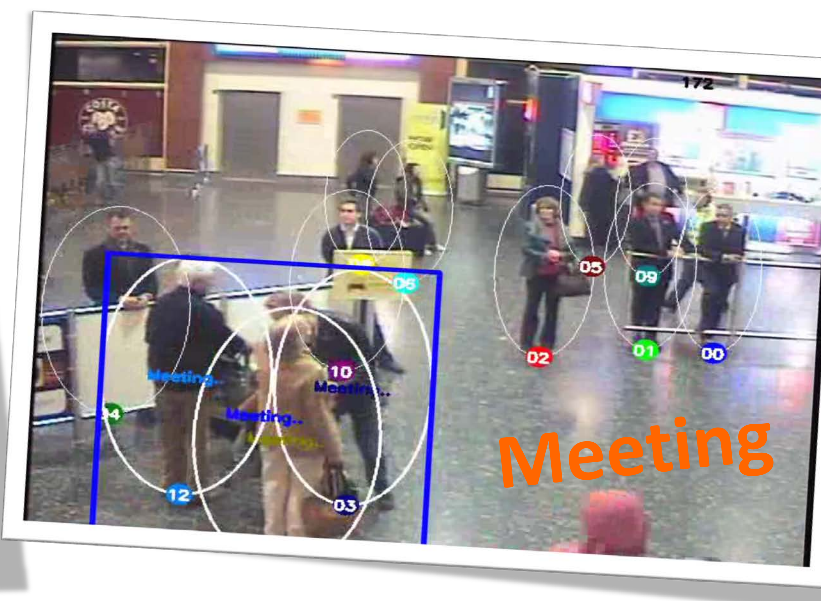
Event Detection
